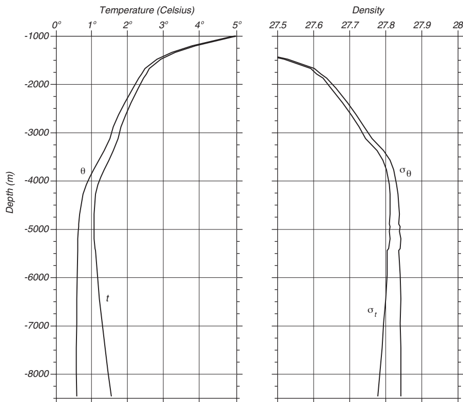
Figure 6.9 Profiles of Left in situ t and potential \theta temperature and Right sigma- t and sigma- \theta in the Kermadec Trench in the Pacific measured by the R/V Eltanin during the Scorpia Expedition on 13 July 1967 at 175.825^\circ E and 28.258^\circ S. Data from Warren (1973).
